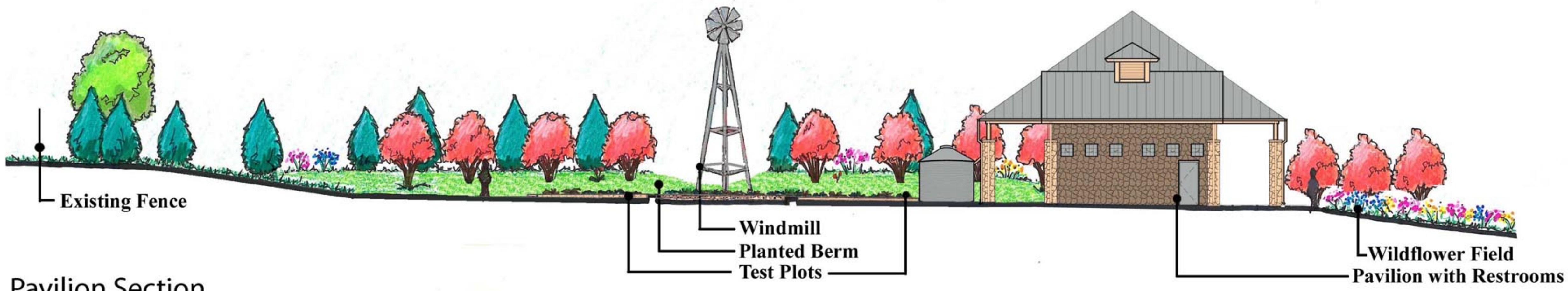
Pavilion Section
